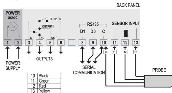
Fig. 2 - N322RHT terminals
