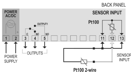
Fig. 03 – Connections on the controller (Pt100 2-wire)
