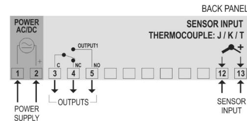
Fig. 04 – Connections on the controller (Thermocouple)
