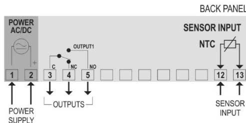
Fig. 01 – Connections on the controller (NTC)
