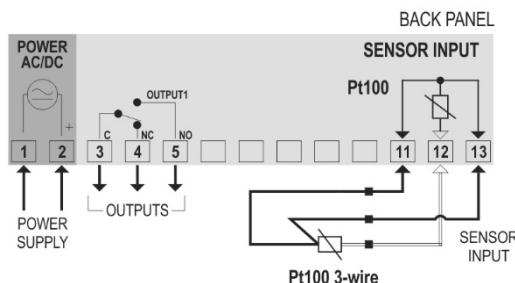
Fig. 02 – Connections on the controller (Pt100 3-wire)
